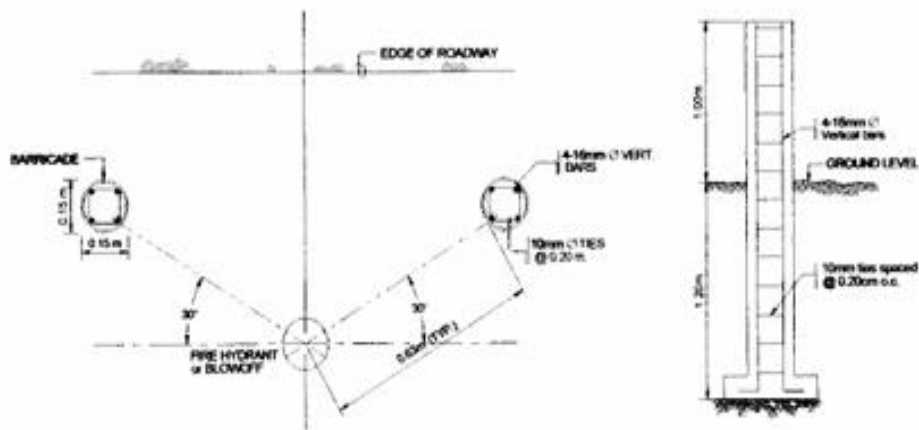
ELEV. OF CONC. BARRICADE
