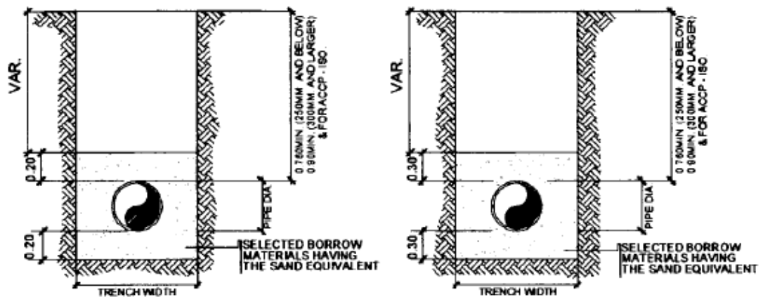
TRENCH DETAILS NOT TO SCALE
