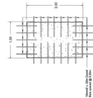
BELLHOLE RESTORATION DETAILS N T S
