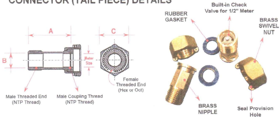
CONNECTOR (TAIL PIECE) DETAILS
