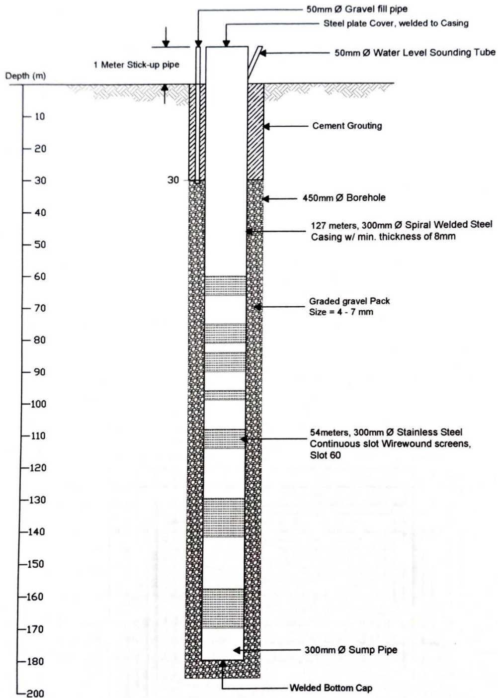
PRELIMINARY WELL DESIGN NOT TO SCALE
