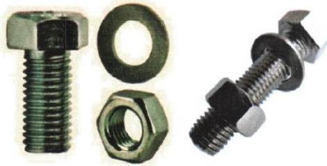
G.I. CAPSCREW 3/4 x 4", full threaded w/ nut and washer, 250 grams
