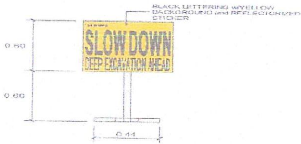
FRONT ELEVATION SCALE 1:25 m
