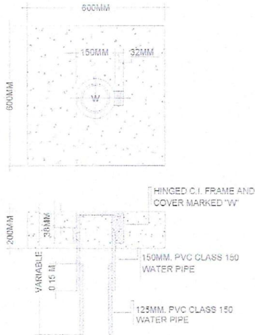
VALVE BOX and COVER DETAIL NOT TO SCALE
