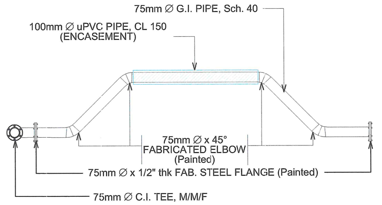
CULVERT CROSSING 3
