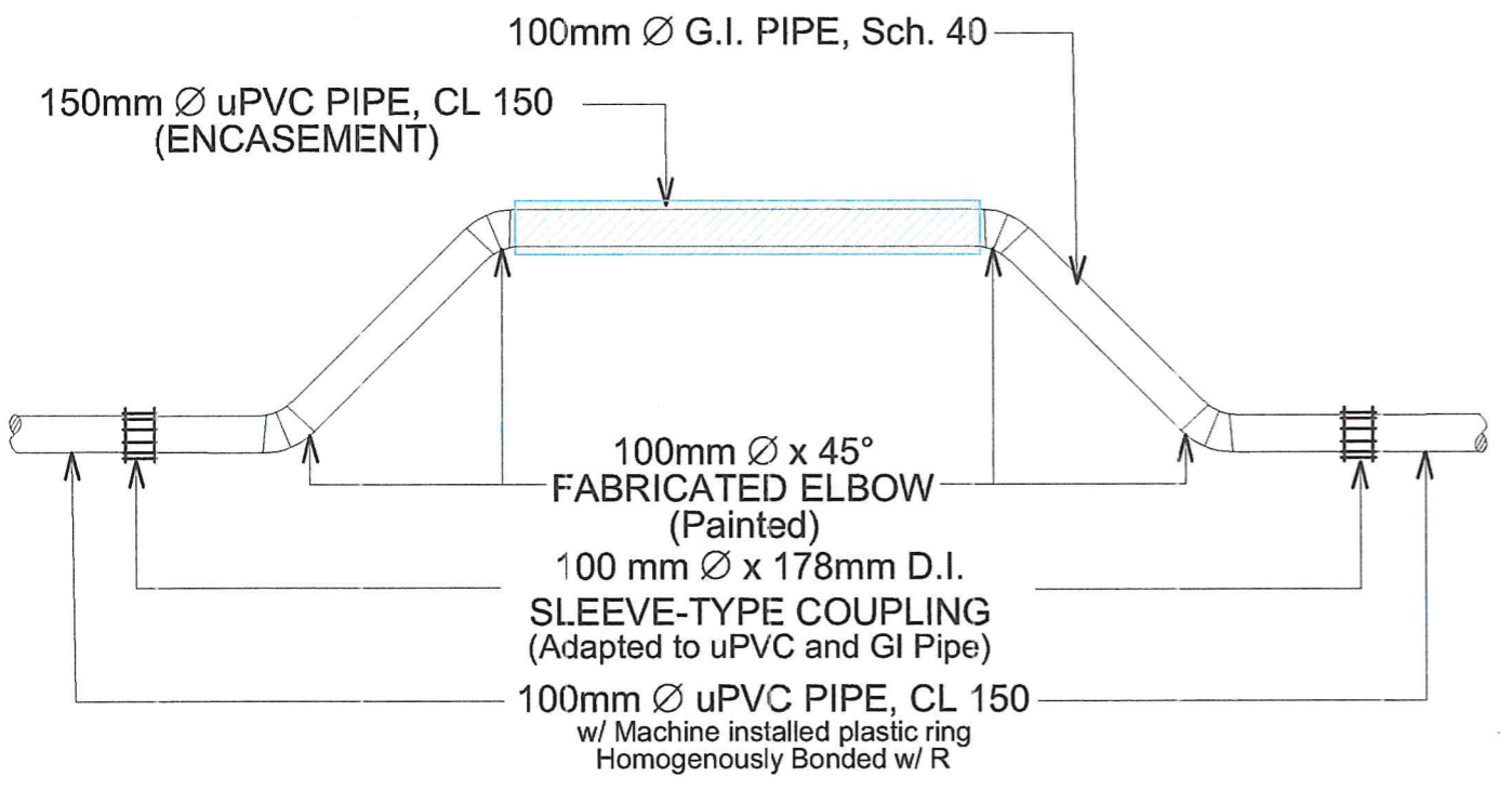
CULVERT CROSSING 1
