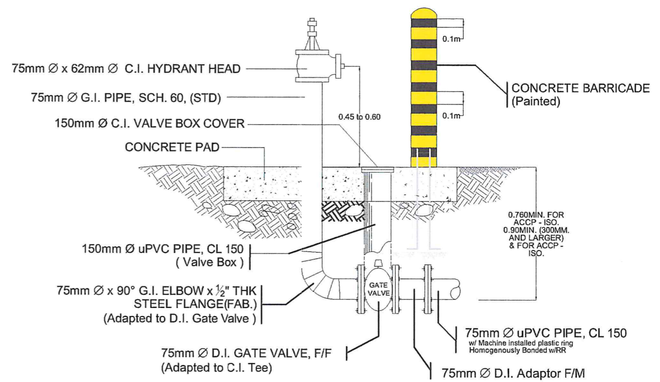
FIRE HYDRANT 3 DETAIL not to scale
