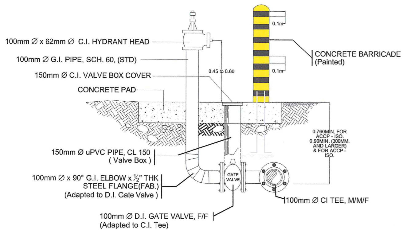
FIRE HYDRANT 1 DETAIL not to scale
