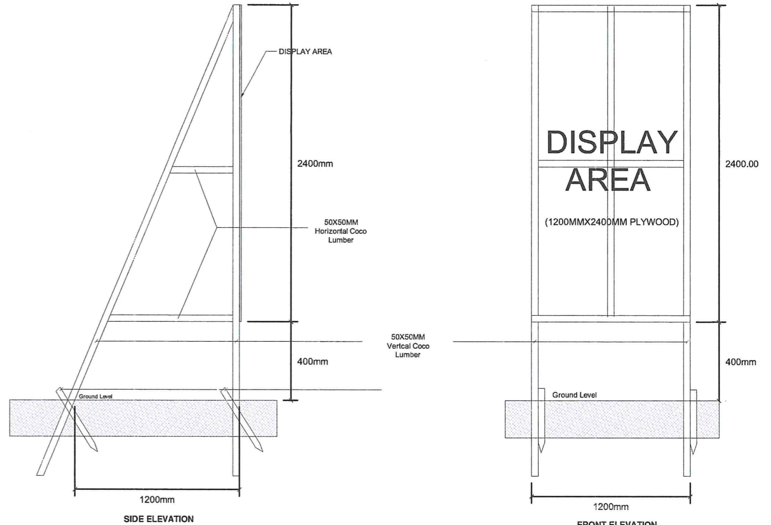
PROJECT BILLBOARD DETAILS not to scale
