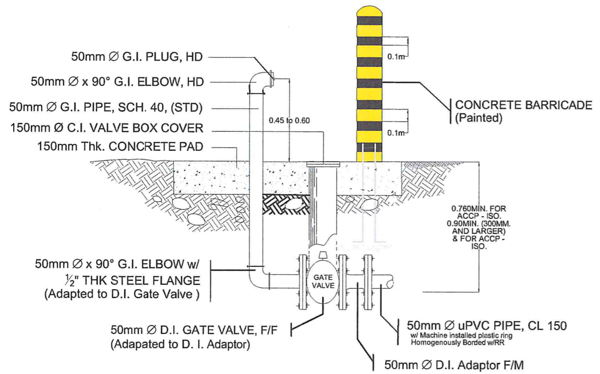
BLOW-OFF 1 and 2 DETAIL not to scale
