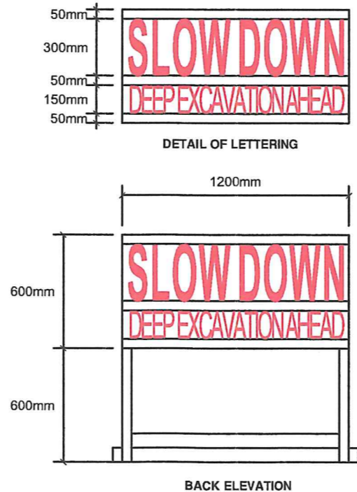
WARNING SIGN DETAIL (WS2) not to scale
