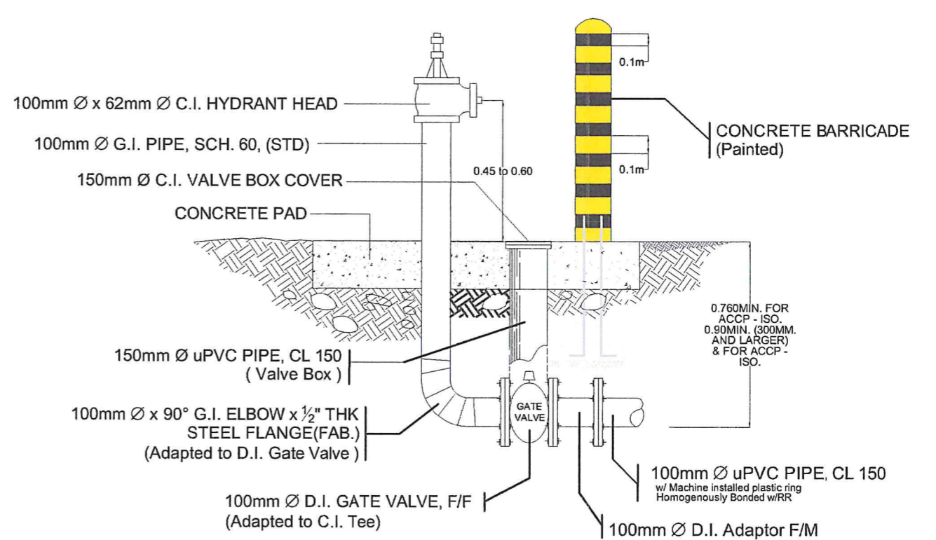
FIRE HYDRANT 2 DETAIL not to scale
