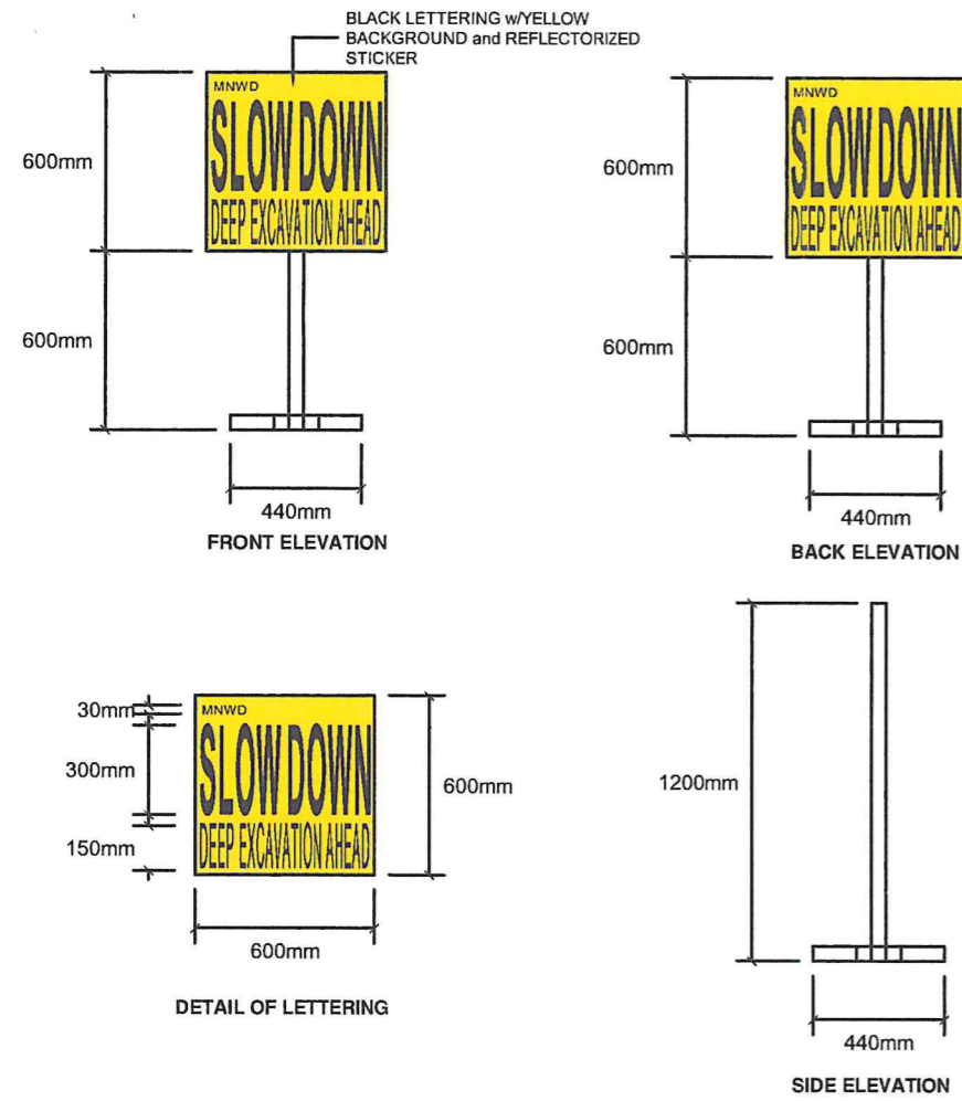
WARNING SIGN DETAIL (WS1) not to scale
