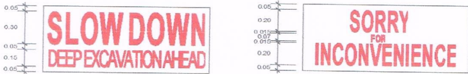
DETAILS OF LETTERING SCALE 1:17.5 m
