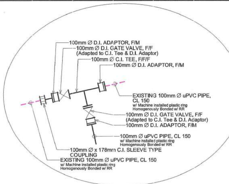
INTERCONNECTION II TO EXISTING WATERLINE DETAIL
