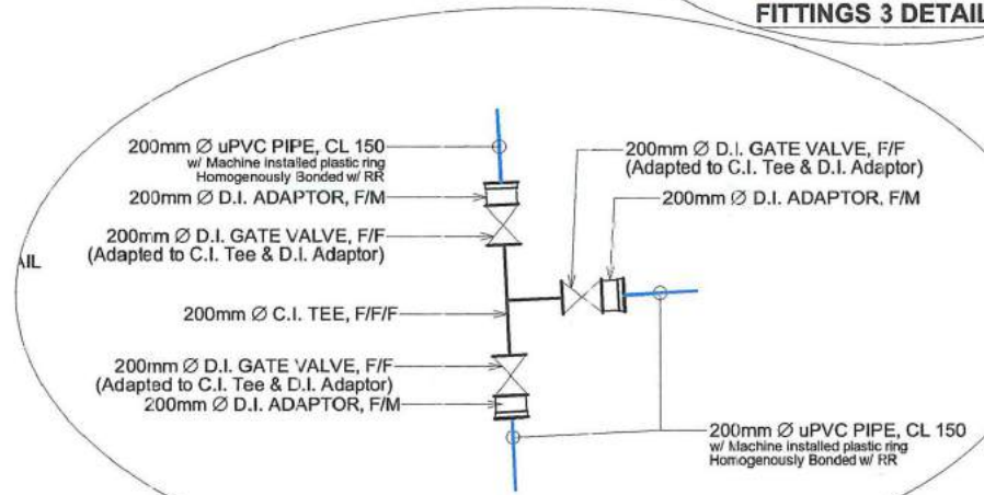
INTERCONNECTION C DETAIL
