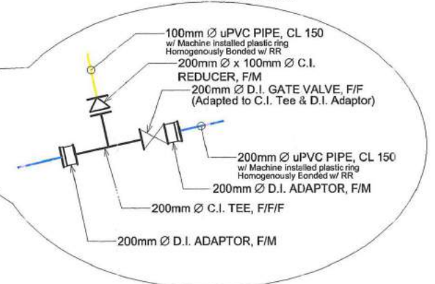
INTERCONNECTION D DETAIL
