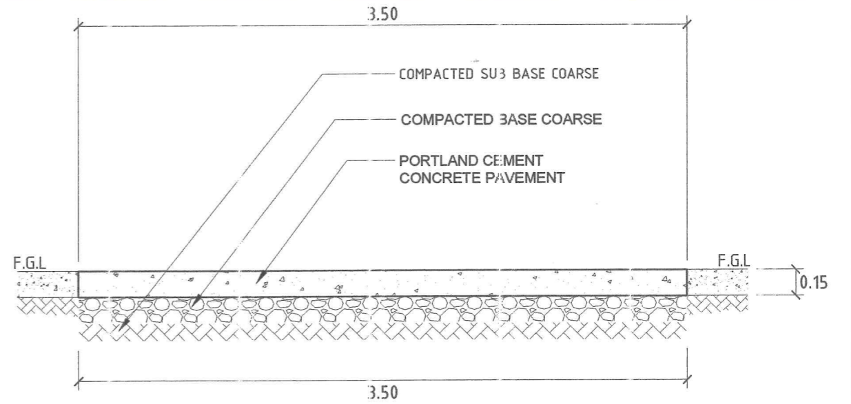
DETAILS OF PCCP
