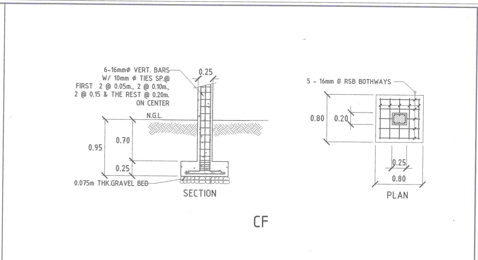
COLUMN/FOOTING DETAILS SCALE : 1 : 40 MTS.
