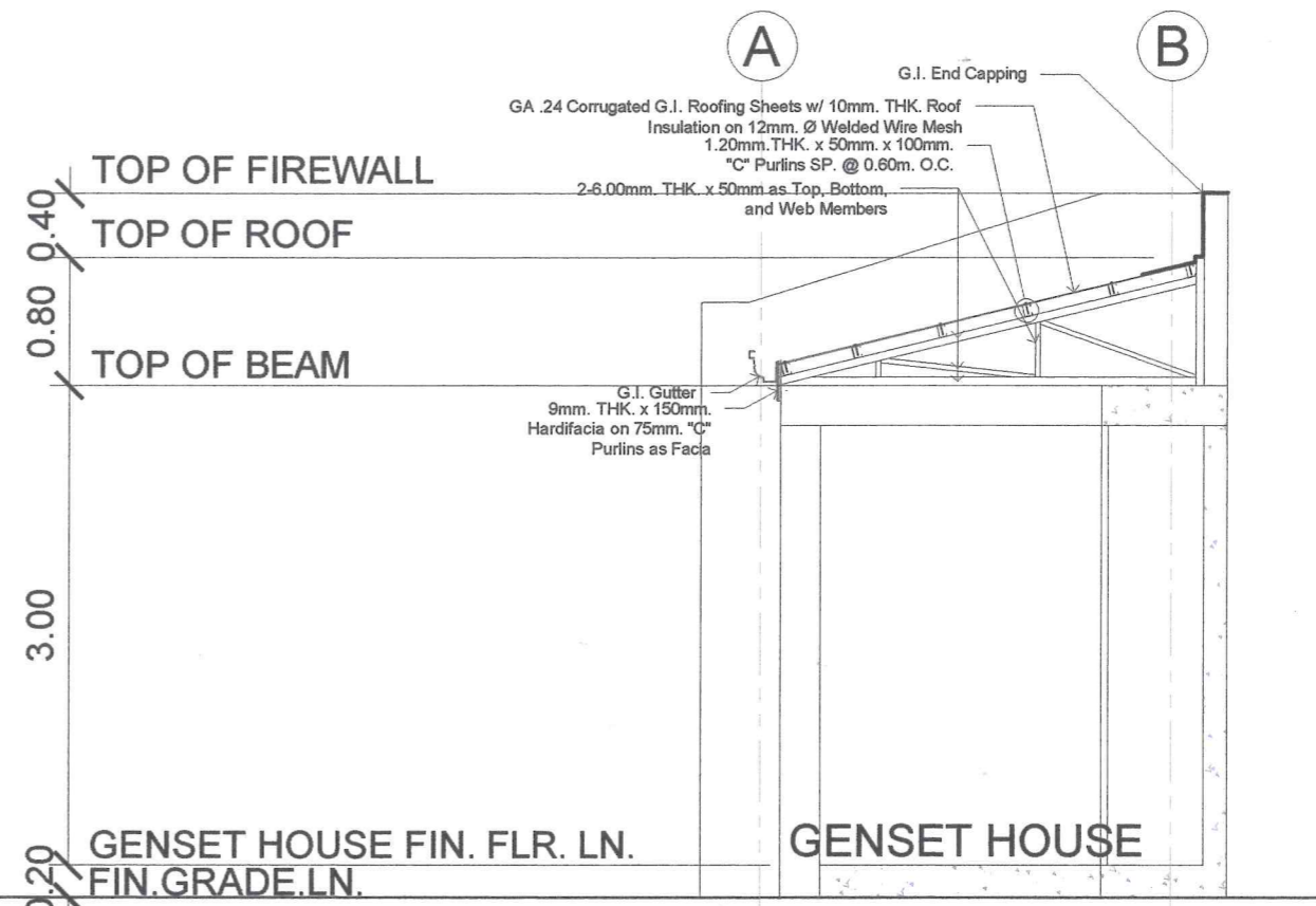
SECTION THRU "X-X" (Genset House)
