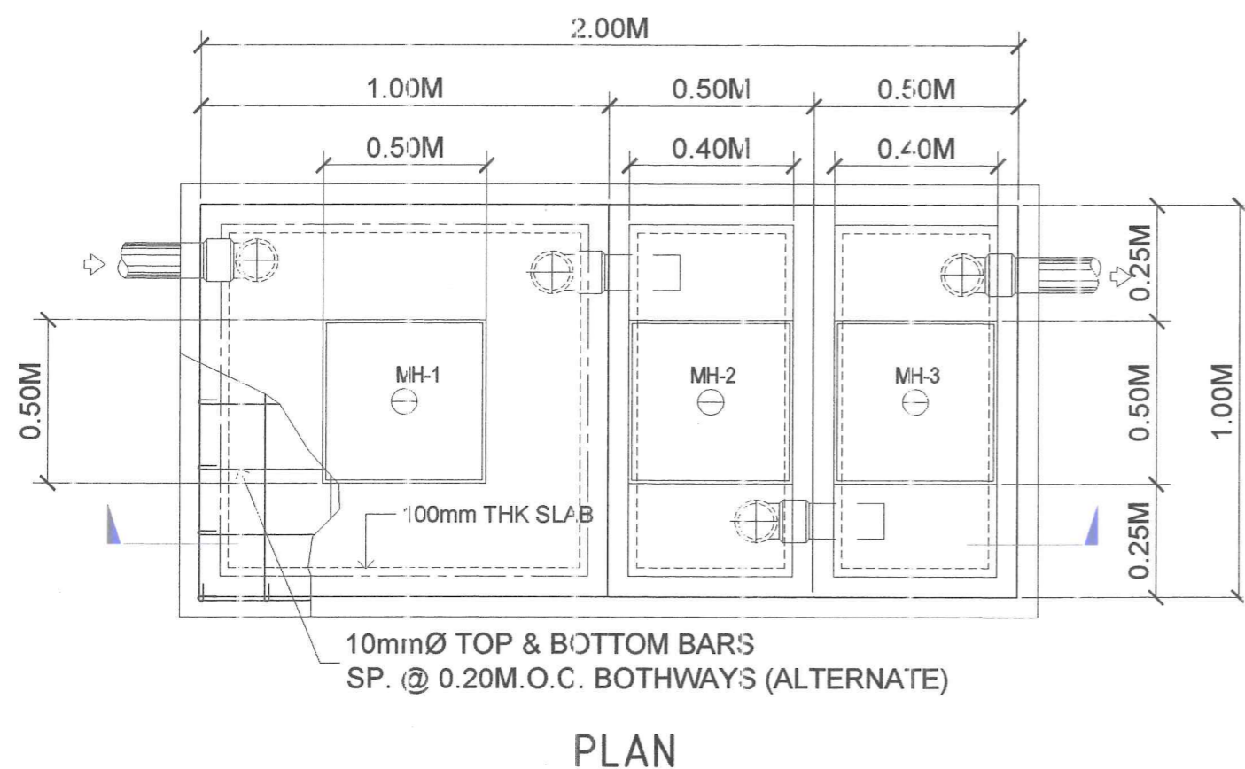
COMFORT ROOM DETAILS
