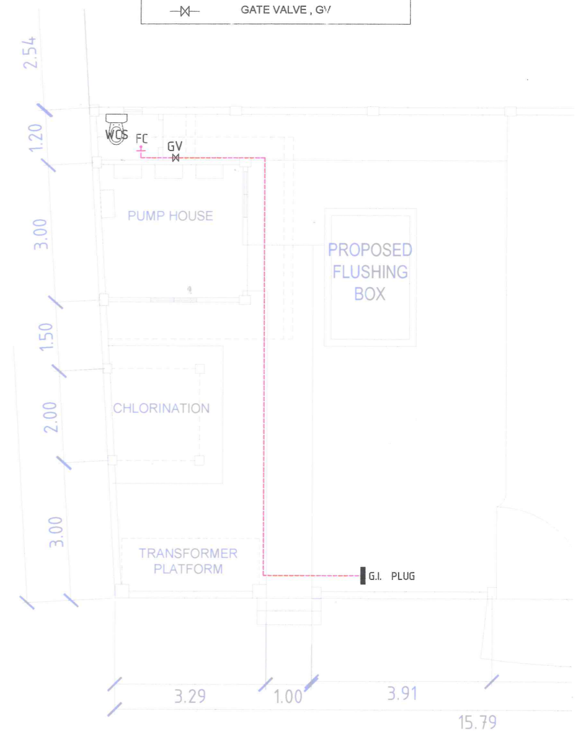
CLEAN WATER LAYOUT
