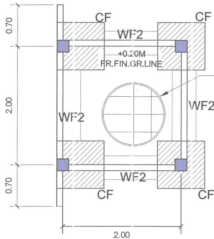
FOUNDATION PLAN
