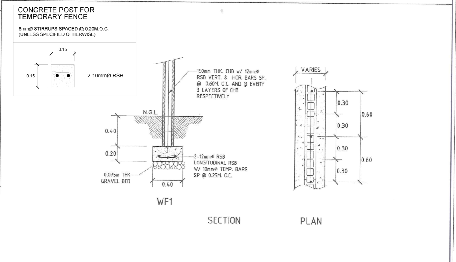
WALL FOOTING DETAILS SCALE : 1 : 30 MTS.
