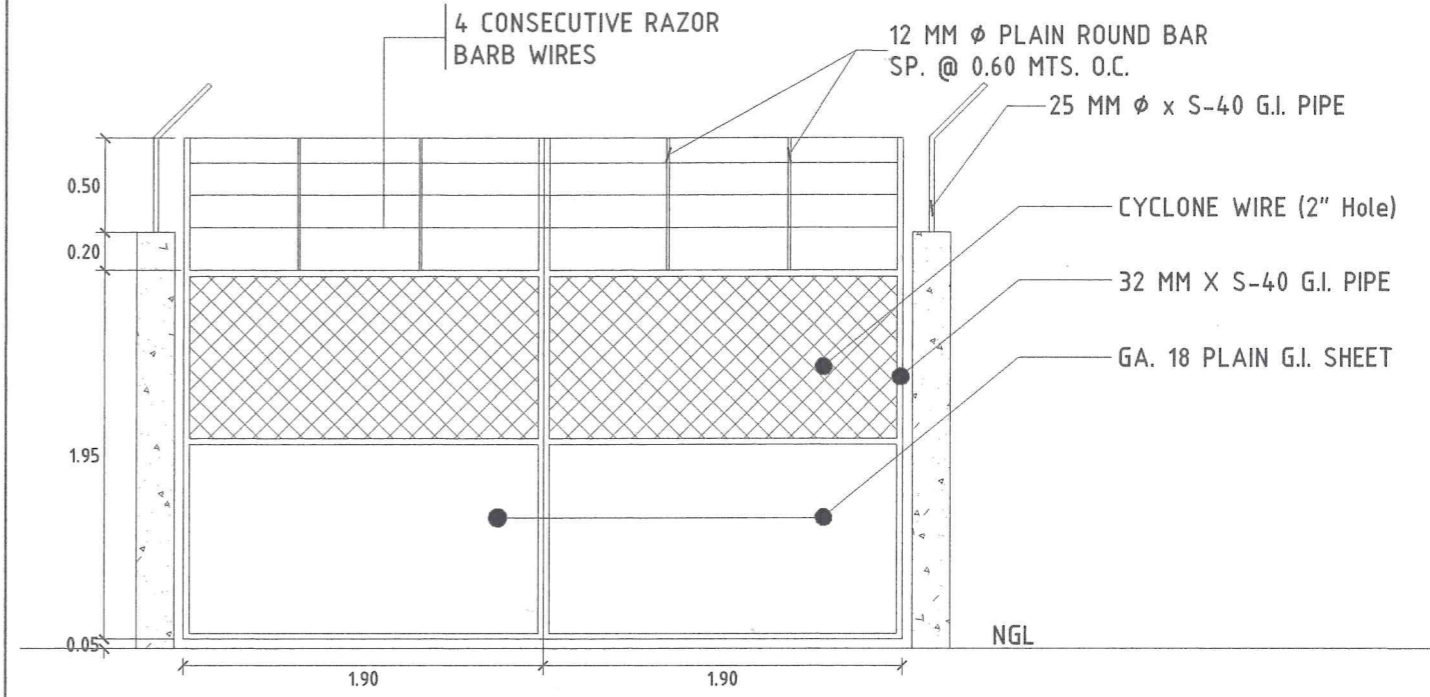
VEHICULAR GATE DETAILS
