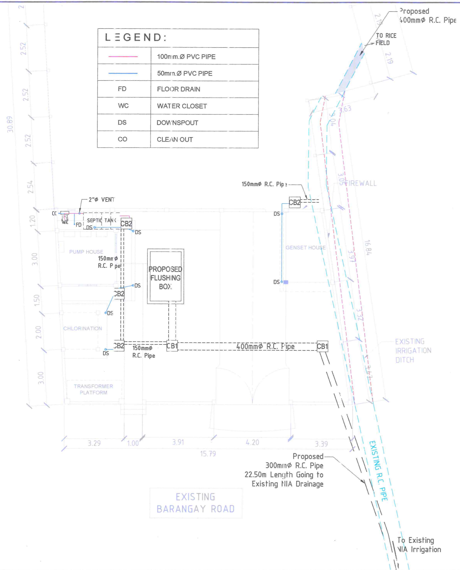
SANITARY LAYOUT
