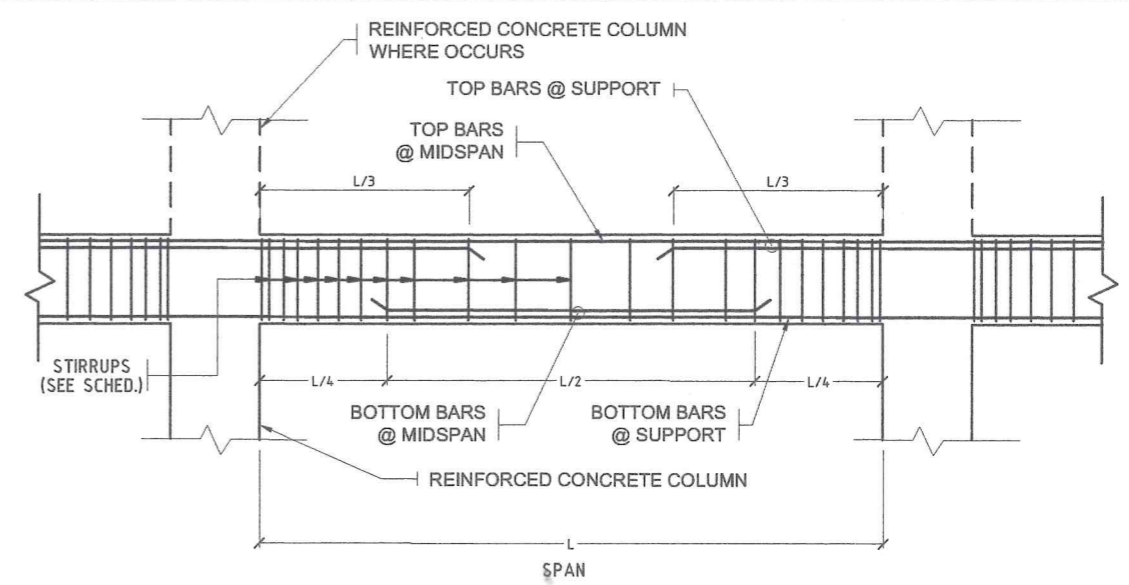
TYPICAL BEAM DETAIL NOT TO SCALE.
