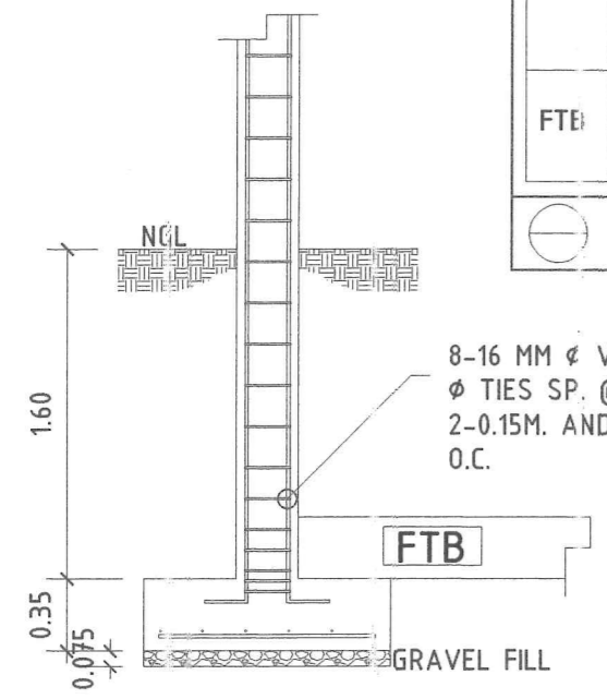
COLUMN FOOTING SECTION
