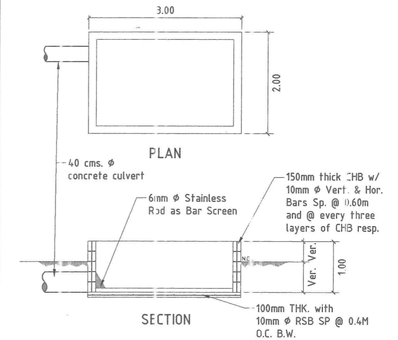
DETAILS OF FLUSHING BOX
