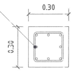
COLUMN PLAN
