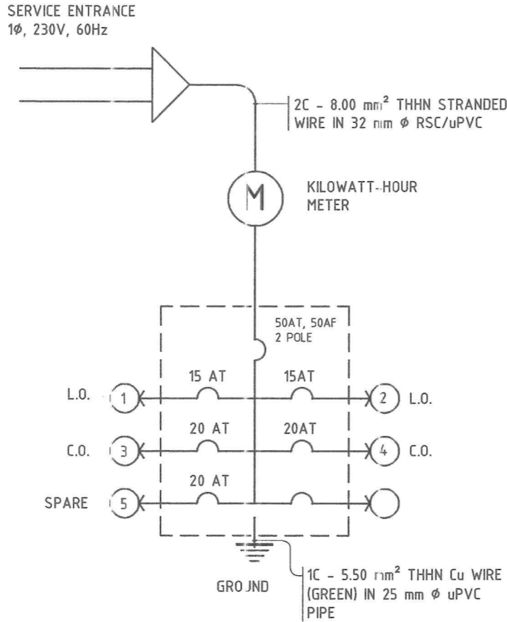
⊕ RISER DIAGRAM SCALE : 1 : 75 MTS.
