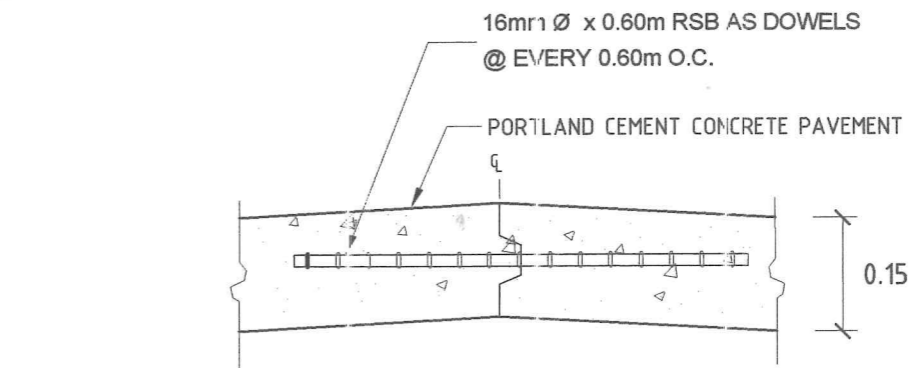
DETAILS OF PCCP
