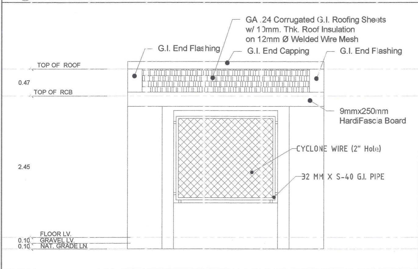
FRONT ELEVATION
