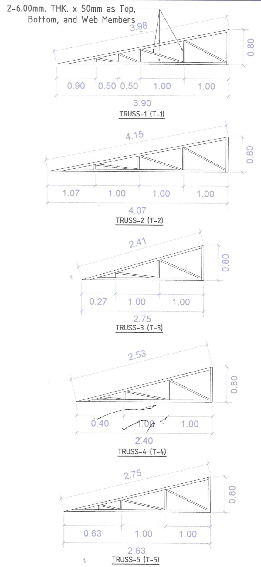
TRUSSES DETAILS N T S
