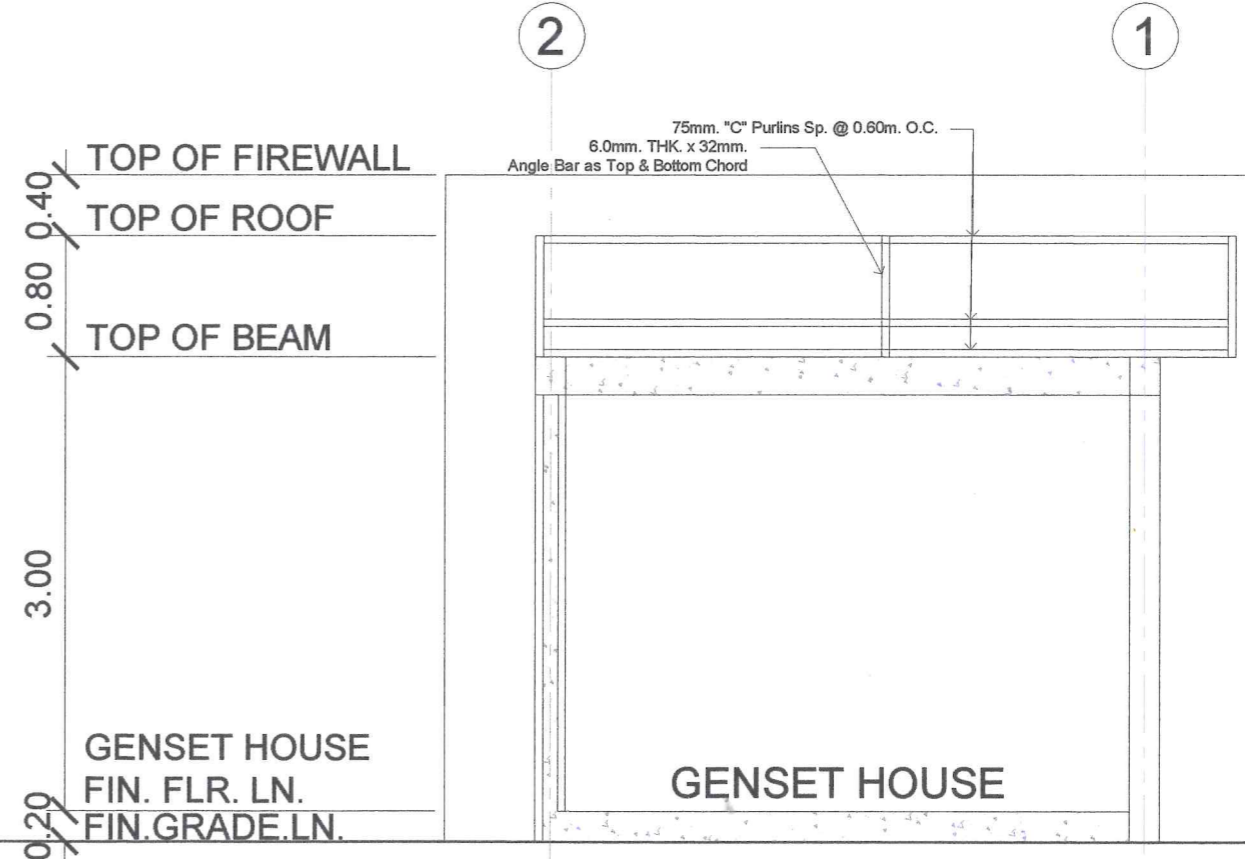
SECTION THRU "Y-Y" (Genset House)
