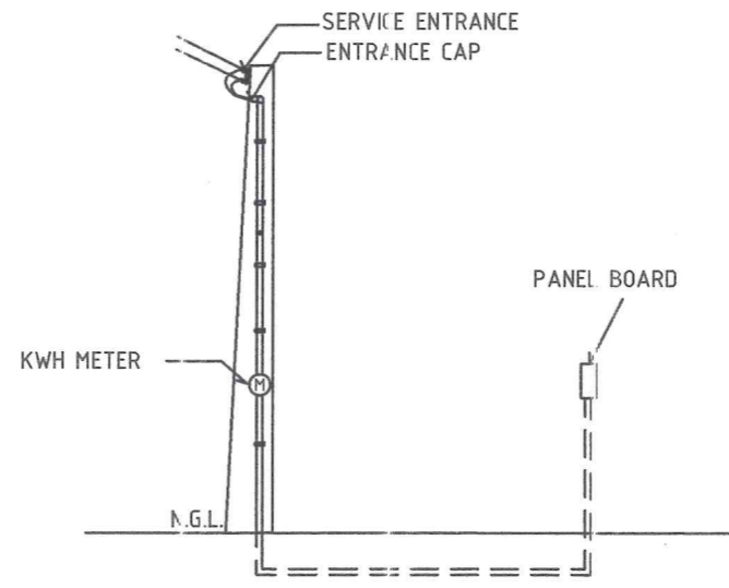
⊕ SERVICE ENTRANCE DETAIL
