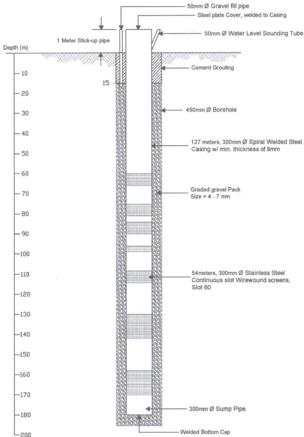
PRELIMINARY WELL DESIGN NOT TO SCALE
